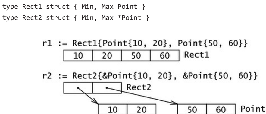
Fig 10.2: Memory layout of a struct of structs
