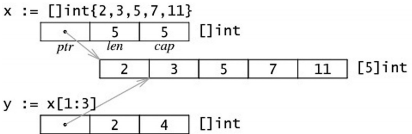
Fig 7.2: Slice in memory
